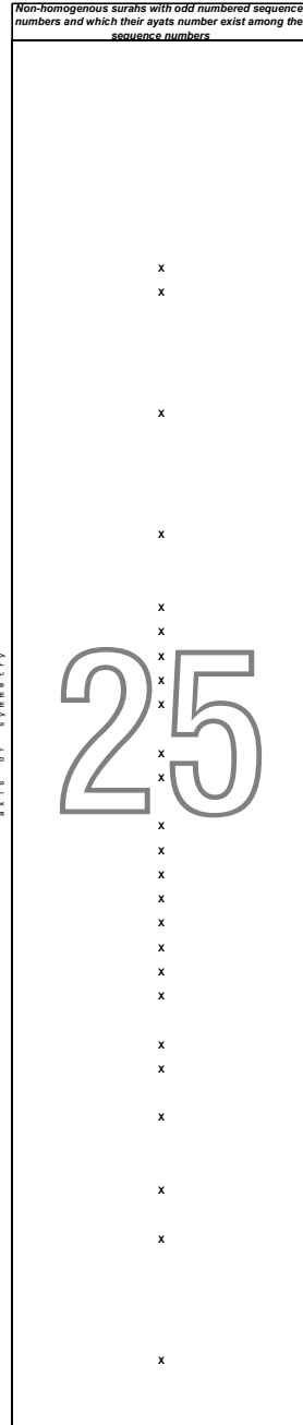
In the figure, equal distribution of the surahs with odd numbered sequence numbers and which their ayats number exist among the sequence numbers is shown.
