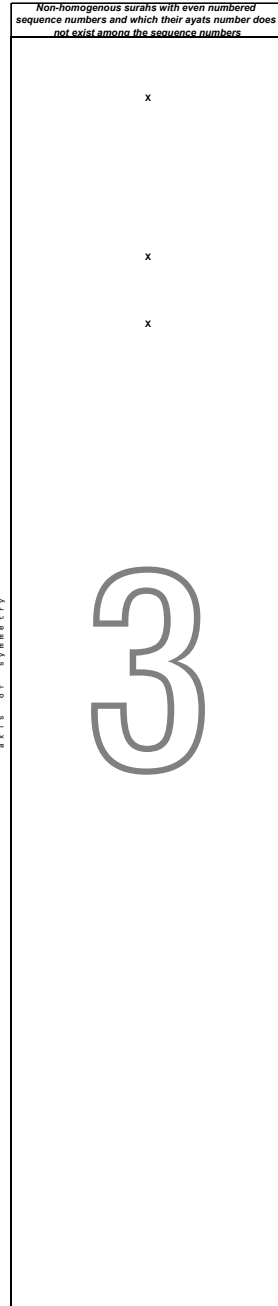
In the figure, equal distribution of the surahs with even numbered sequence numbers and which their ayats number does not exist among the sequence numbers is shown.
